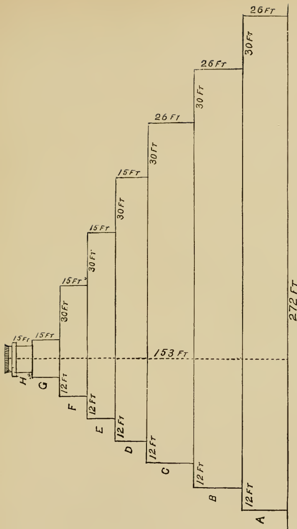
70.—PLAN OF THE ZIGGURAT OF BORSIPPA (BIRS-NIMRUD). (Rawlinson.)
